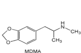
MDMA
