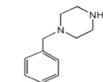
1-Benzylpiperazine (BZP)
