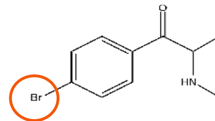
4-Bromo-methcathinone (4-BMC)
